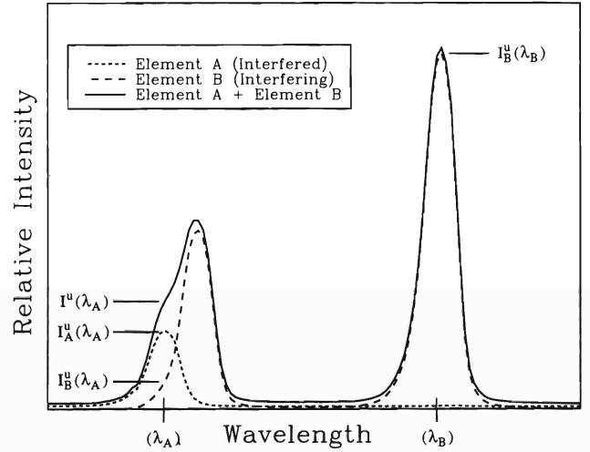
FIGURE 1. Schematic diagram showing a hypothetical spectral interference.
